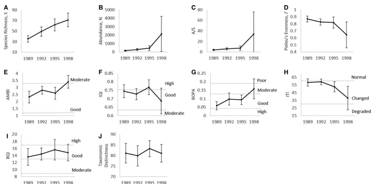
Fig. 5. Change in macrobenthic community indices over time at Ironotter Point (Firth of Clyde, UK) (average across all sites with standard deviation, 1989 N = 64, 1992 N = 66, 1995 N = 84, 1998 N = 14). 1989 was the baseline year, before implementation of the sewage outfall pipe. Note that AMBI, A/S and BOPA have inverse relationships with quality. For details of indices, see Table 1. Quality classification threshold information can be found in Table S2.
