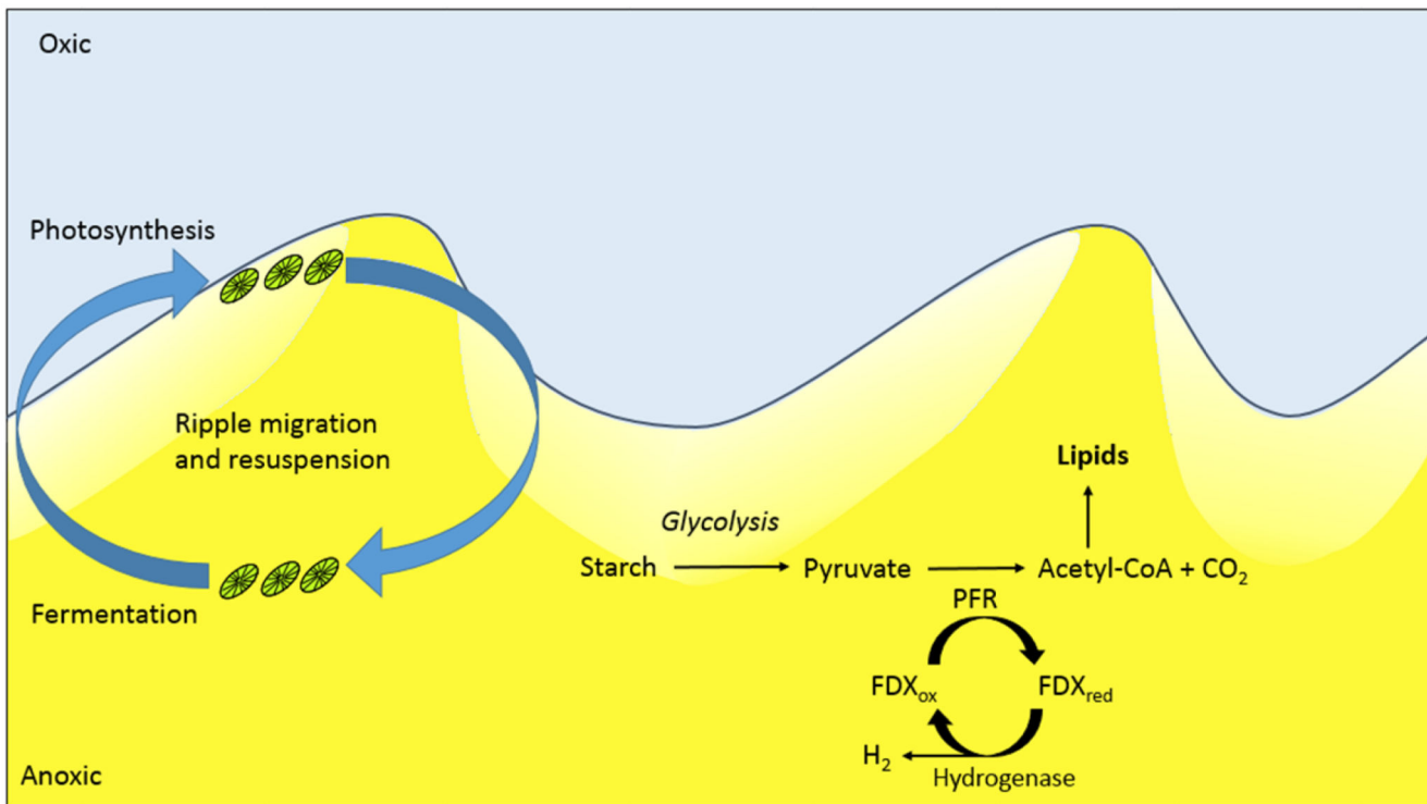
Figure 3. Conceptual model of benthic algal metabolism in sand sediments. In this energetic environment, ripple migration and sediment resuspension regularly move algal cells many centimetres into the sediment where it is dark and anoxic. Under these conditions, microalgae undertake dark fermentation associated with high rates of H_2 and lipid production 25. Enzyme designations are pyruvate ferredoxin oxidoreductase (PFR) and ferredoxin (FDX). Lightly shaded areas represent declining oxygen concentration within the sediment. Yellow shaded area represents anoxic permeable sediment.
