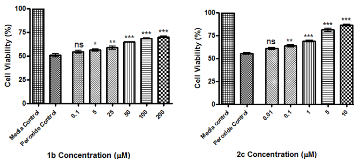
Figure 2. Protective effects of compound 1b and 2c in hydrogen peroxide ( 400\mu\text{M} )-stressed cells. Cells were incubated with 1b ( 0.1\text{-}200\mu\text{M} ) or 2c ( 0.01\text{-}10\mu\text{M} ) for 24 hours before the addition of hydrogen peroxide. After 24 hours the cell viability was measured using the MTT assay. Values are expressed as the percentage of the untreated control and represented as mean \pm SD of three independent experiments in each group. *** p < 0.001 , ** p < 0.01 , * p < 0.05 , ns no significantly different compared to the control.
