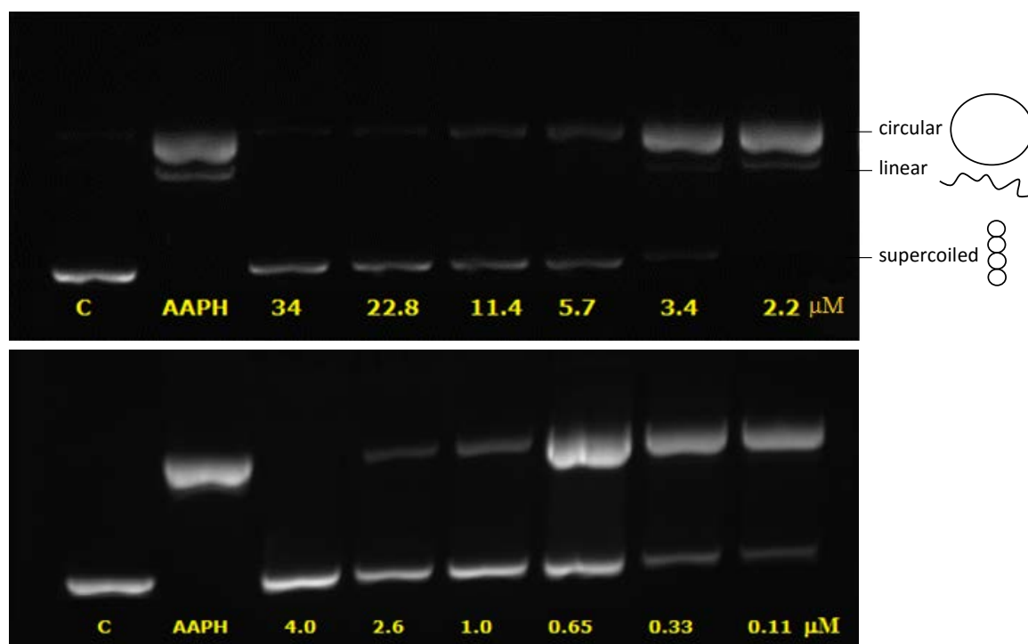
Figure 1. Gel image obtained after DNA protection assay for vanillin (above) and compound 2c (below). The first band (c) at the base represents the DNA control; the band (AAPH) is the AAPH control, the bands from (34 – 2.2 μM) and from (4.0 – 0.11 μM) represent the DNA protection for different concentrations of the compounds. The intensity of each band was measured with image J software and the percentage of protection was measured for each concentration.
