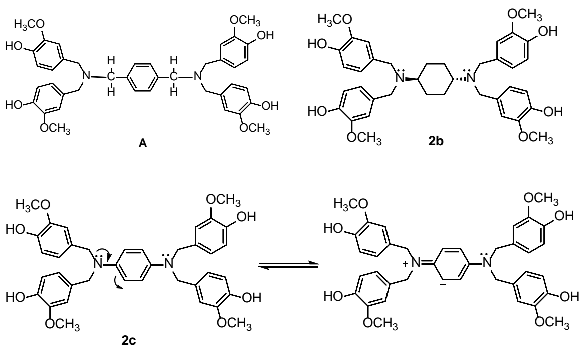
Figure 4. Benzyl Vanillin derivative, A [19] and Phenyl Vanillin derivatives, 2b and 2c . The nitrogen's electron pairs cannot be delocalized in the cyclic system nearby (compound A and 2b ). However, delocalization is possible for compound 2c .
