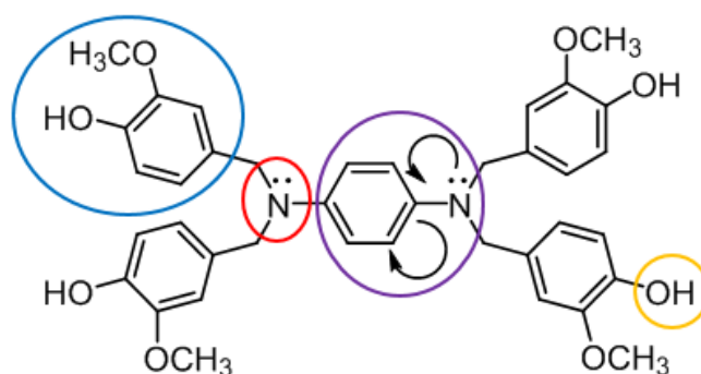
Figure 3. SAR study for new derivatives. The key features for the antioxidant activity are highlighted in different colours: vanillin moiety (blue), phenolic functionality (yellow), tertiary amine (red) and electronic delocalisation (purple).
