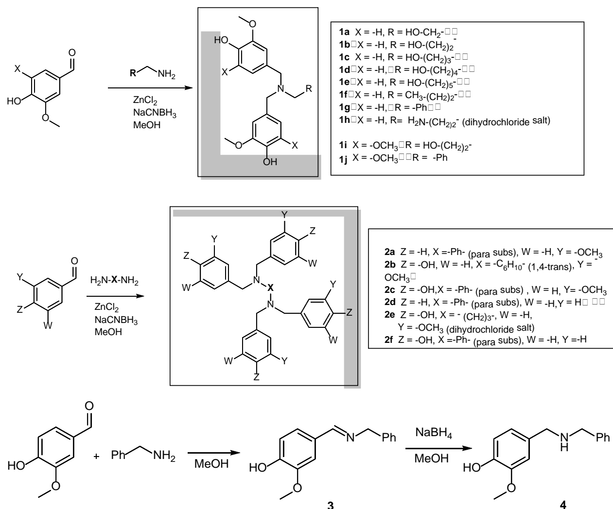
Scheme 1. Chemical strategy for the synthesis of Vanillin derivatives
