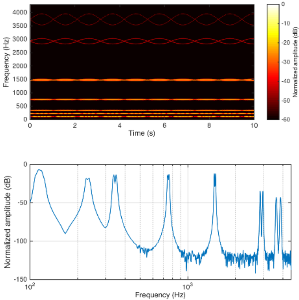
Figure 2: The upper panel shows the spectral output evolution for the simulated tidal turbine signal over a 10 second period (FFT length 4096, 50% overlap, \Delta f = 10.76 Hz, sample rate of 44100 Hz). The lower panel is a ‘snap shot’ FFT part way through the 2.1 second frequency modulation cycle (FFT length 8192, \Delta f = 5.38 Hz, sample rate of 44100 Hz). The amplitude of each tonal component is normalized to the equivalent broadband source level. The amplitude ratio here is compensated for the relative transmit sensitivity of the transmitter transducer representing the relative ratios the levels in the water.
