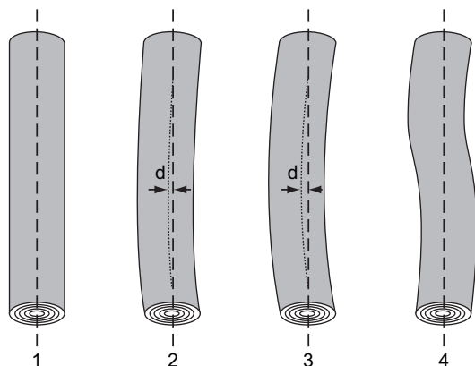
Figure 1. Specification for log straightness (after Forestry Commission, 1993). Logs 1 and 2 qualify as straight logs; logs 3 and 4 do not qualify. Maximum deviation ( d ) on log 2 does not exceed 1 cm over 1 m length. Maximum deviation ( d ) on log 3 exceeds 1 cm over 1 m length. Log 4 shows bow in more than one direction.
