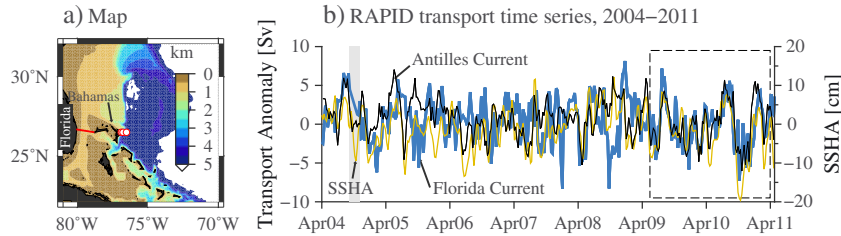
Figure 1. (a) Map of the region with land in black and bathymetry shaded at 500 m intervals. Moorings used to estimate the AC transport are given by the red open circles, WB 2 and WB 3 at 76.75°W and 76.5°W, respectively, and 26.5°N. Additional moorings used are between WB 2 and the Bahamas and are indistinguishable at this scale. The SSH anomaly time series at 76.67°W and 26.5°N are between the centers of the two visible white dots. The FC cable position is given by the red line between Florida and the Bahamas islands. (b) Florida Current (thick blue) and Antilles Current transport anomalies (thin black) for the period April 2004 to April 2011, with amplitudes on the left y axis. Also plotted are SSH anomalies at 26.57°N, 76.67°W, with the seasonal cycle removed (yellow). The roughly 2 month period from September to October 2004 is shaded in grey indicating a gap in the FC cable data. The box (black, dashed) shows the period where the FC and AC are correlated.
