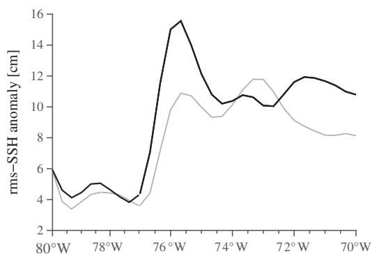
Figure 4. Root mean square amplitude of SSH anomalies along 26.58^{\circ} N for the intervals April 2004 to April 2009 (solid grey line) and May 2009 to April 2011 (solid black line), as in Kanzow et al. [2009, Figure 6].
