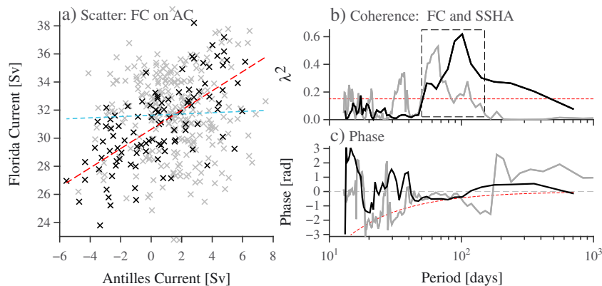
Figure 2. (a) Scatter plot of transport time series for the FC and AC, for April 2004 to April 2009 (grey) and May 2009 to April 2011 (black), with the best fit regression lines in blue and red, respectively, and correlation coefficients r=0.04 (not significant) and r=0.66 (99% significant), respectively. (b) Magnitude squared coherence between the FC transport and the SSH anomaly time series, for the same periods, and colors as in Figure 2a. Areas above the red, dashed curve are significant. The box (dashed black) indicates the mesoscale timescales (50–150 days). (c) Phase in radians, where a 7 day lag (SSH leading) is in dashed red.
