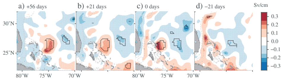
Figure 3. Lagged regression maps between the AC transport and SSH anomalies for the time period May 2009 to April 2011, where the SSH time series has had its seasonal cycle removed. The slope of the regression is plotted in color for lags of (a) 56, (b) 21, (c) 0, and (d) -21 days. Positive lags indicate that the SSH anomalies precede the AC transport anomalies. Significant regions at the 95% level are contoured in black. The 800 m bathymetric contour is also contoured with dashed grey.
