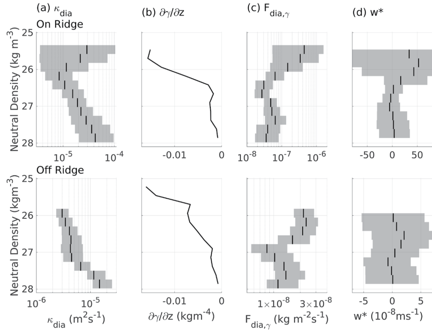
Figure 4. The diapycnal advection for the on-ridge (upper row) and off-ridge (lower row) stations. The profiles: (a) diapycnal diffusivity, \kappa_{dia} ( m^2s^{-1} ), (b) vertical density gradient, \partial\gamma/\partial z ( kg\ m^{-4} ), (c) the diapycnal diffusive flux of density, F_{dia,\gamma} ( kg\ m^{-2}s^{-1} ), positive directed towards denser surfaces, and (d) diapycnal advection, w^* ( m\ s^{-1} ), positive directed upwards. The black lines show the mean values derived from the microstructure data and the cruise-observed gradients. The shaded regions indicate 95% confidence ranges using a bootstrap method.
