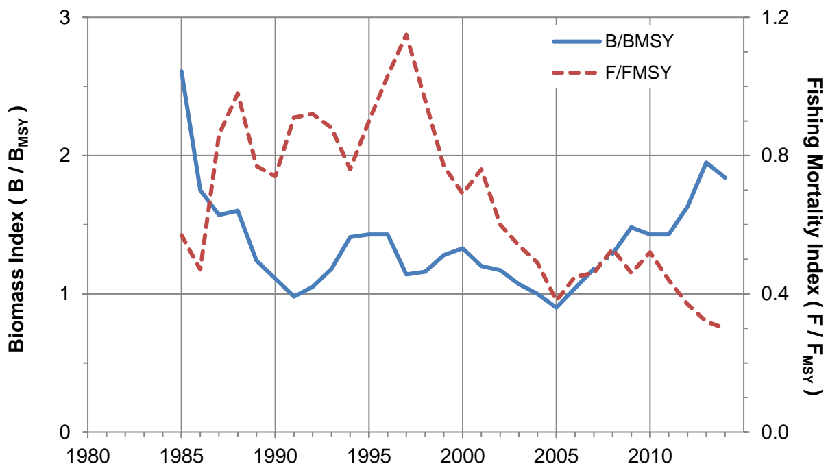
Figure 7 Indices of the biomass and fishing mortality rate of the North Sea and West of Scotland megrim stock from 1985 to 2014.
